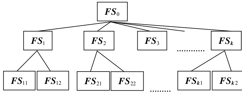
Figure 1. Structure of the control system.
