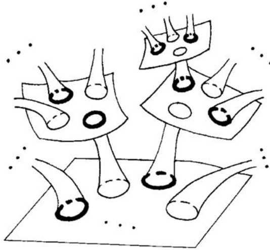
Fig. 2.1. The surface R for \chi(S) \leq -2
